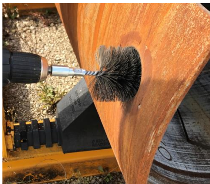
Illustration 1: Cleaning brush in operation
